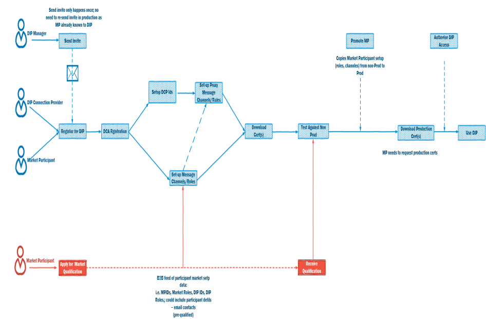
Figure 7 – On-Boarding Steps
